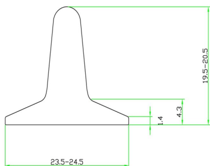
20mm high T cleat
