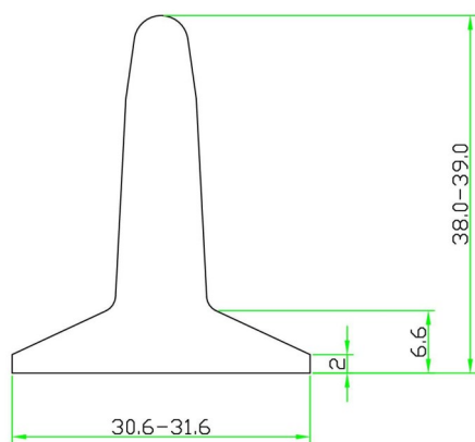
38mm high T cleat
