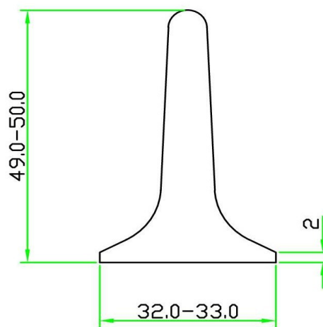
50mm high T cleat
