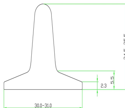
25mm high T cleat
